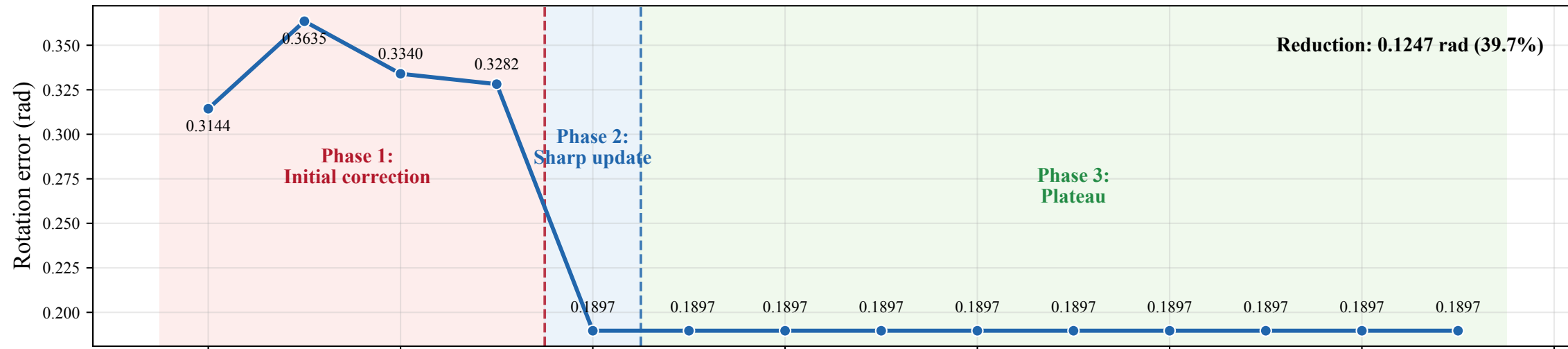
Rotation Error vs Outer Iteration
